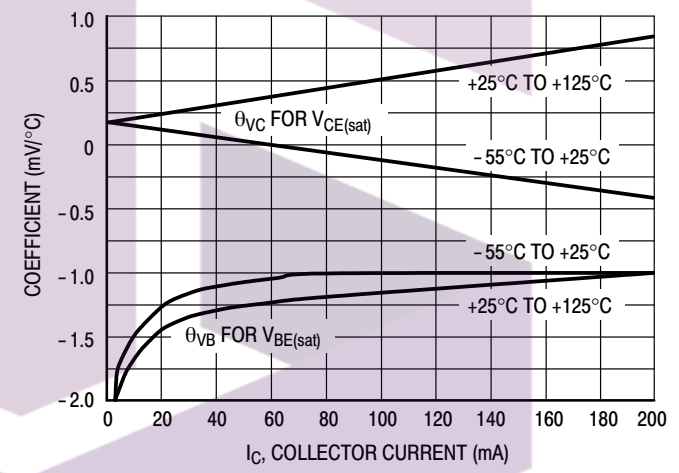
Figure 20. Temperature Coefficients
