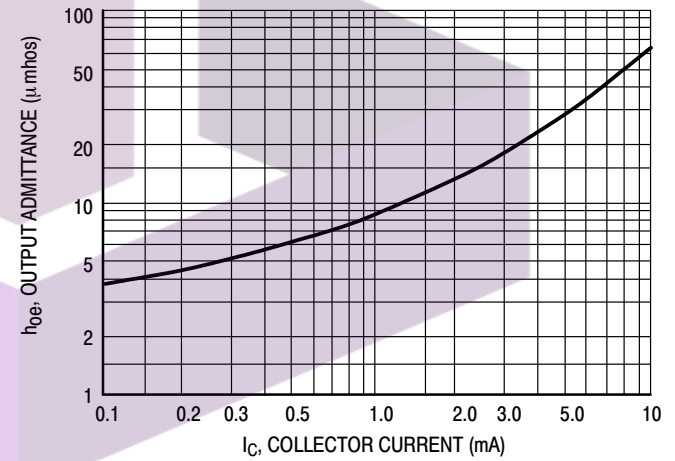
Figure 12. Output Admittance
